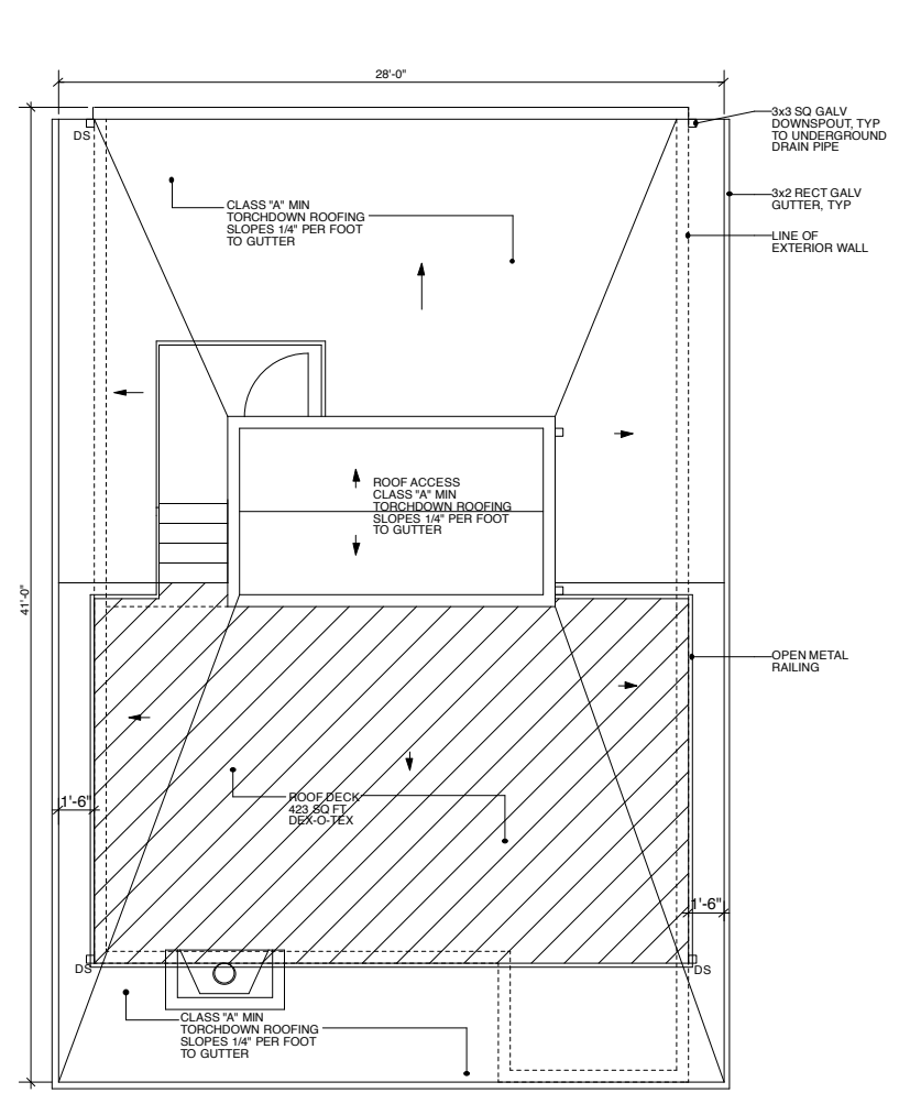
UNIT 1 ROOF PLAN 3
