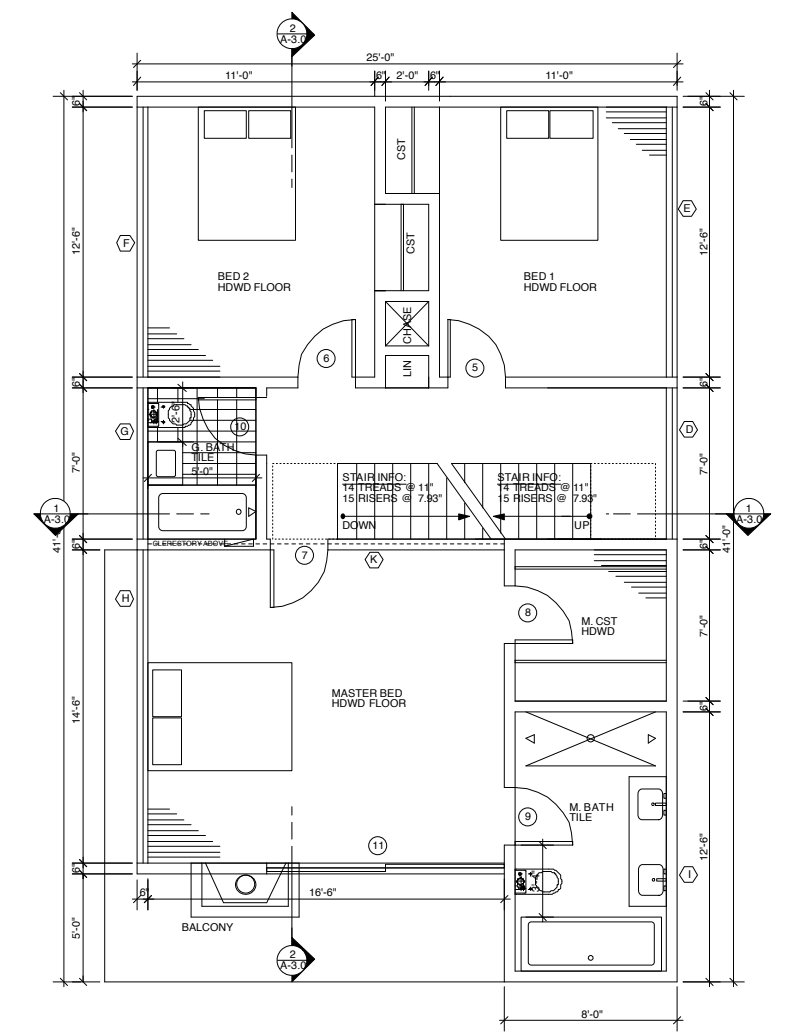
UNIT 1 2ND FLOOR PLAN 2
