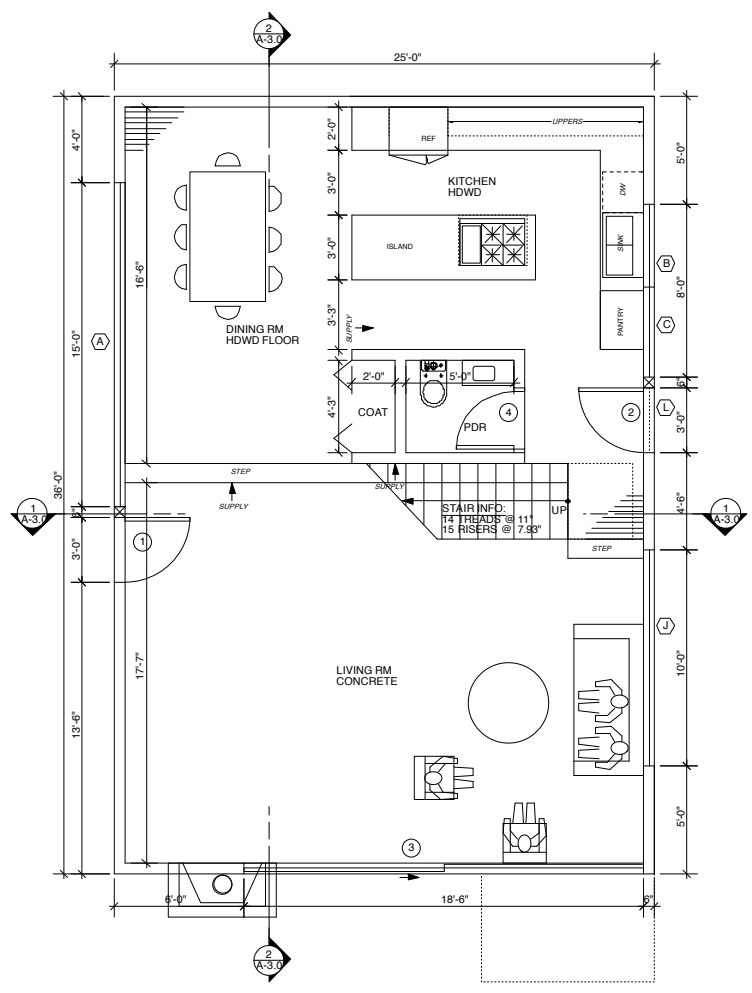
UNIT 1 1ST FLOOR PLAN 1
