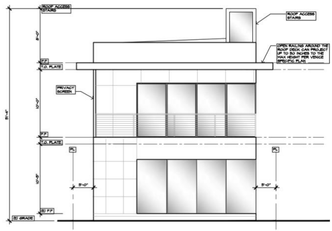
2 PROPOSED NORTH ELEVATION 3/16" = 1'-0"
