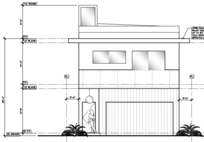
1 PROPOSED SOUTH ELEVATION 3/16" = 1'-0"
