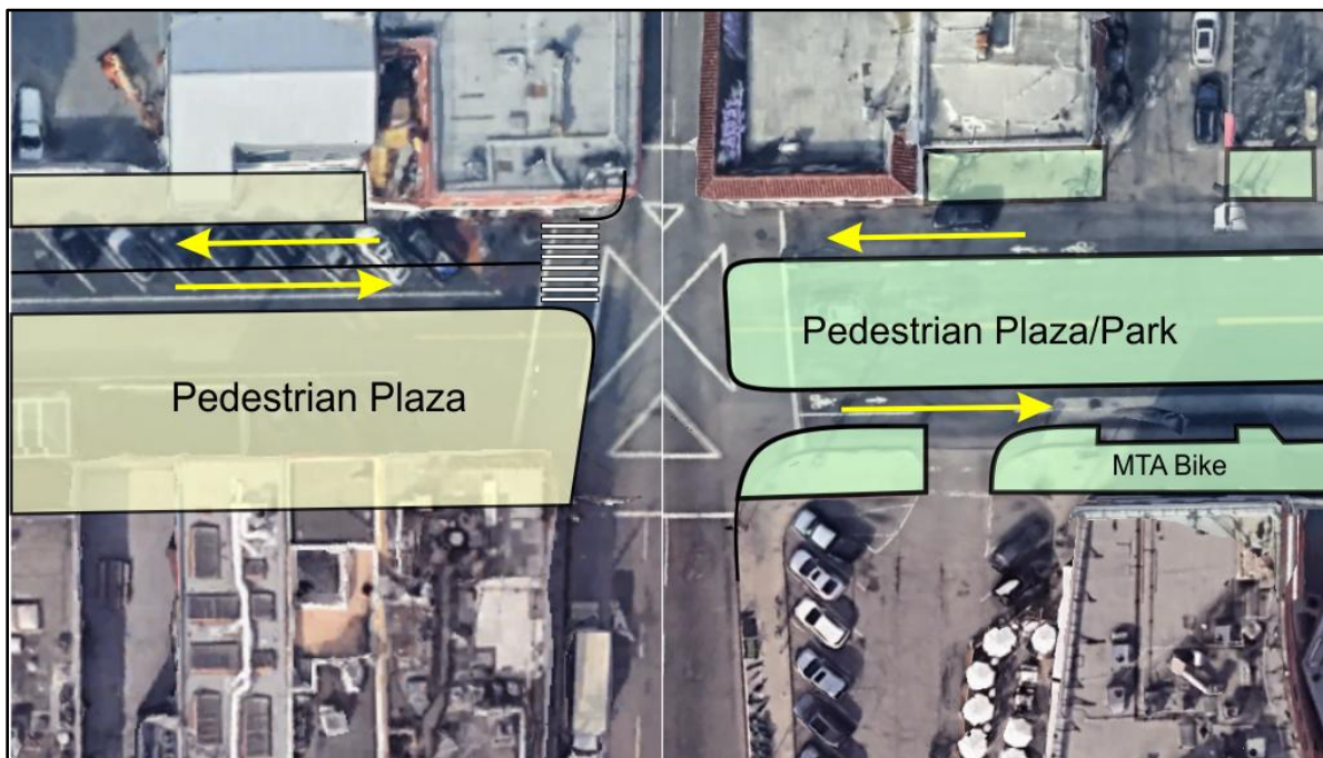
Figure 8: The Intersection of Pacific Avenue and Windward Avenue with Concept 2
