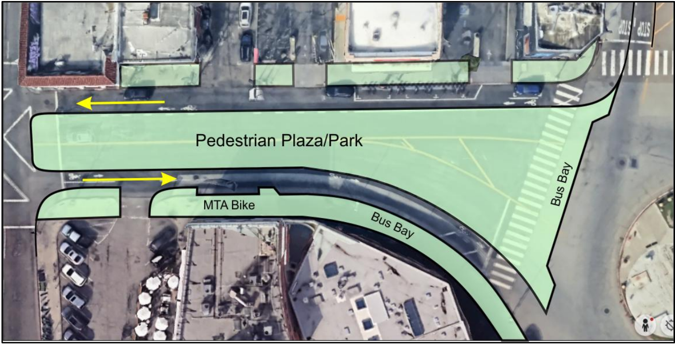
Figure 6: Concept 2 for Reconfiguring Windward Avenue Between Pacific Avenue and Windward Circle
